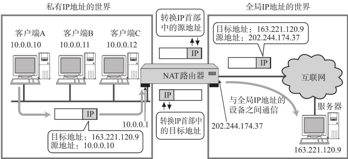
图5.19 NAT
