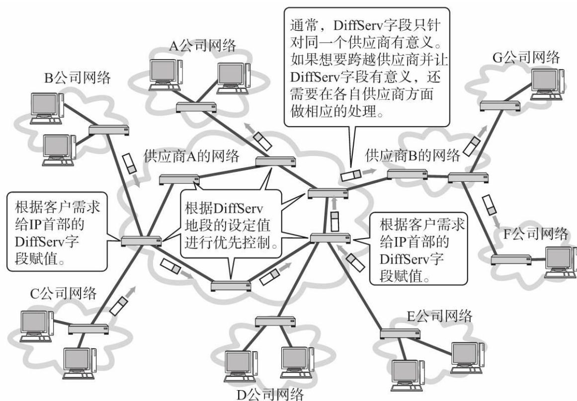
图5.28 DiffServ
