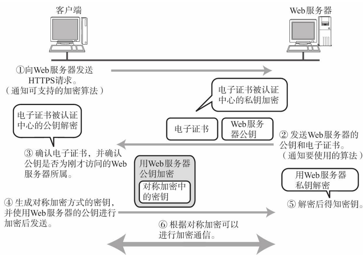
图9.8 HTTPS
