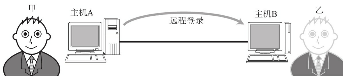
图2.15 TELNET
