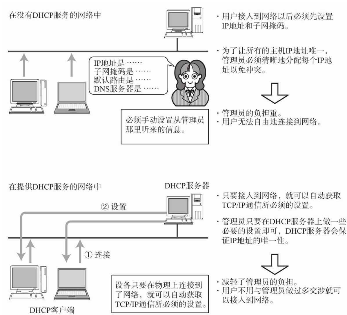
图5.16 DHCP
