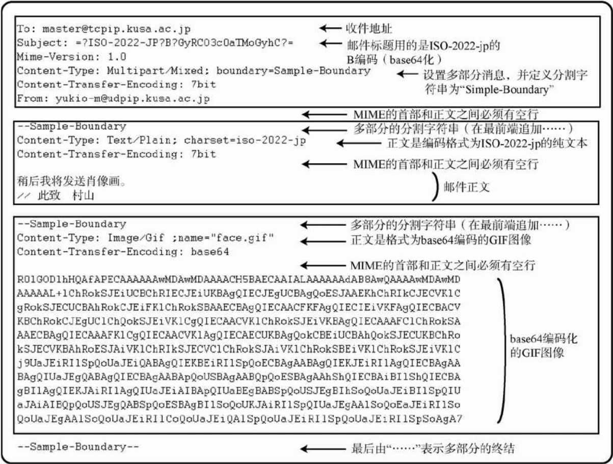
图8.11 MIME举例
