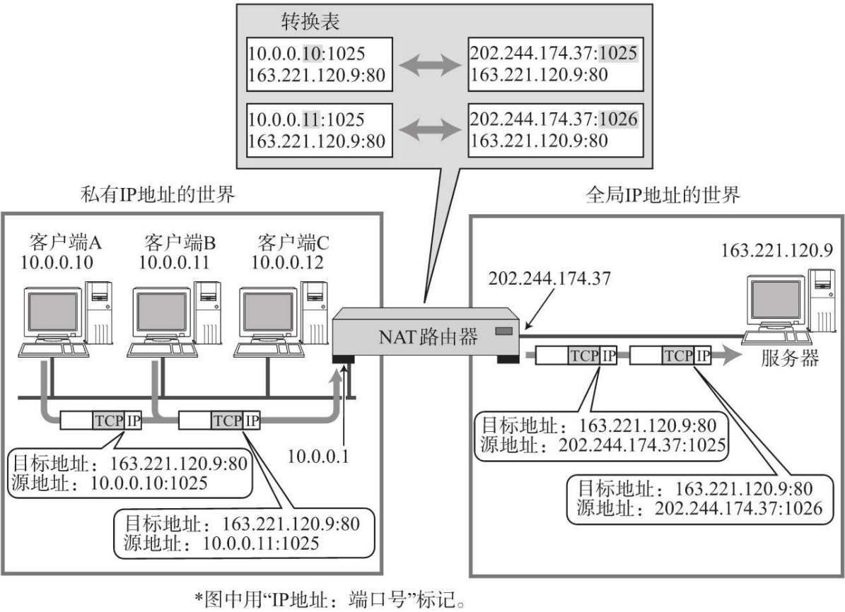
图5.20 NAT
